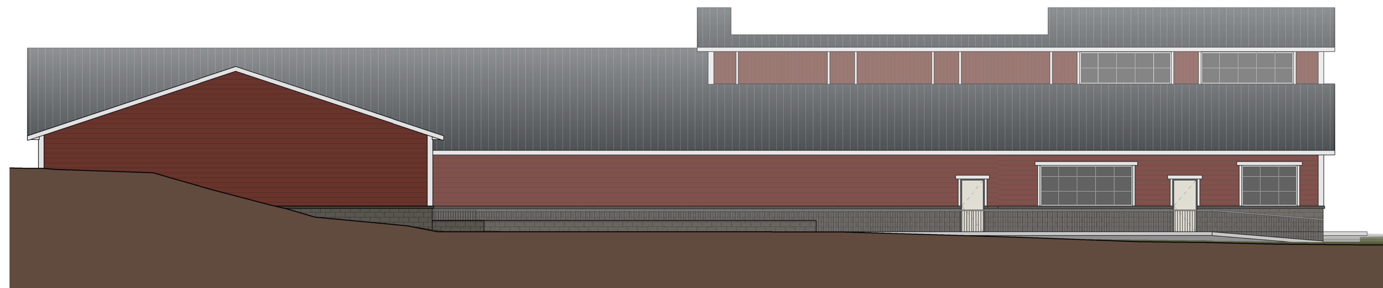
3 NORTH ELEVATION 1/8" = 1'-0"
