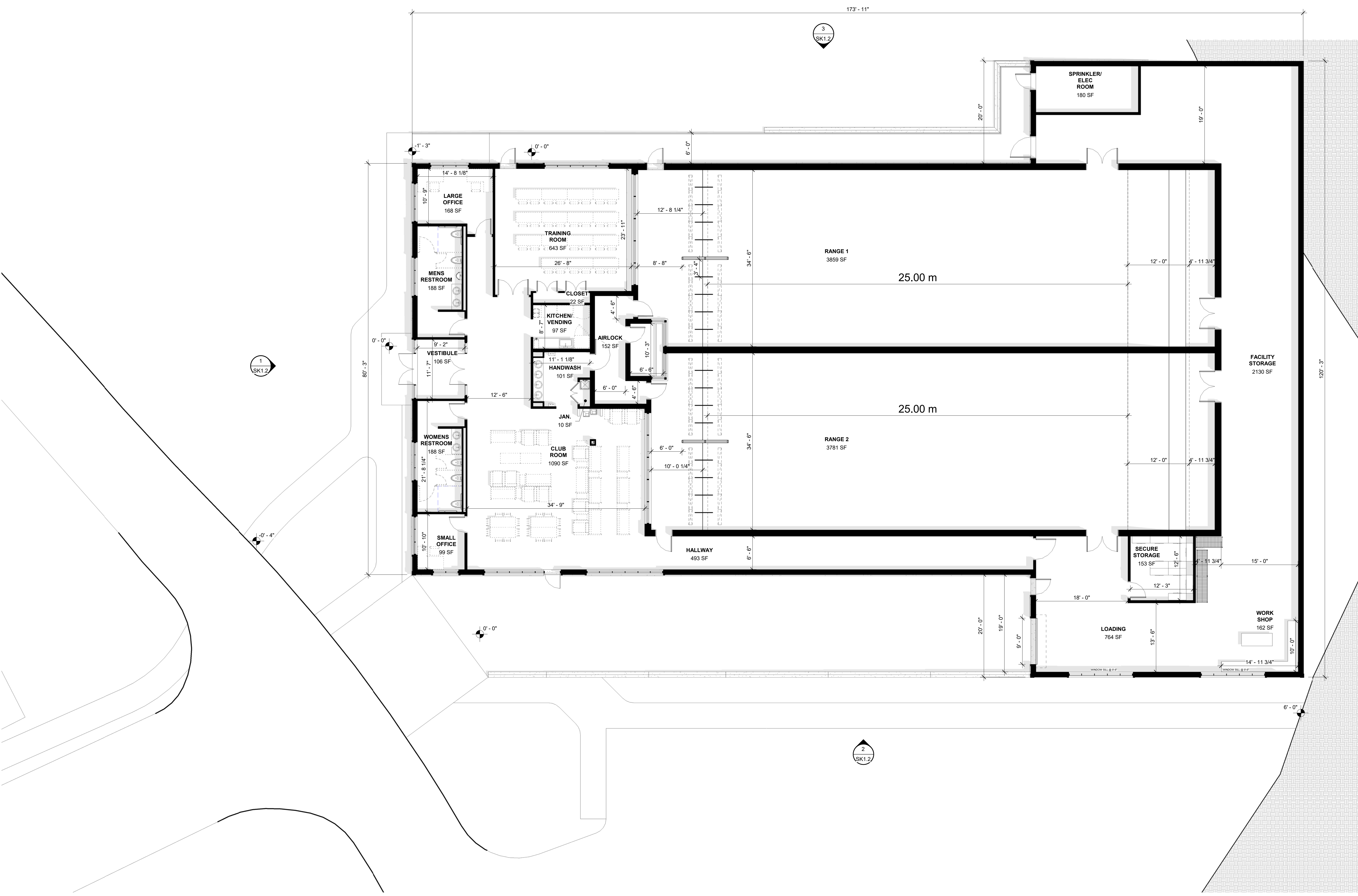
1 FLOOR PLAN 1/8" = 1'-0"
